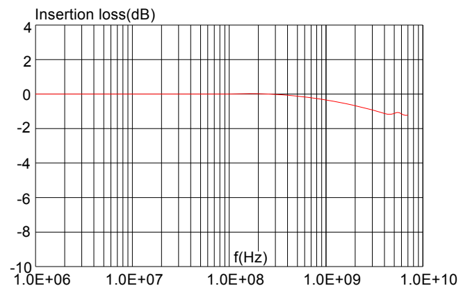
FIG.6: Insertion loss S21 of I/O to GND
