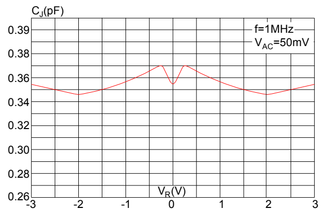
FIG.8: LTP measurement
