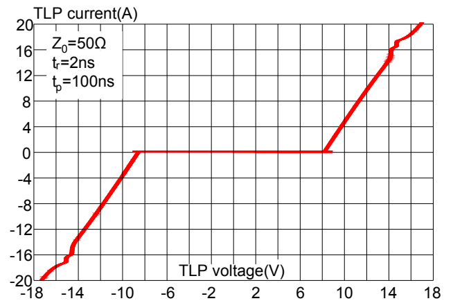
FIG.6: TLP Measurement
