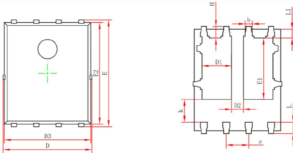
Top View
