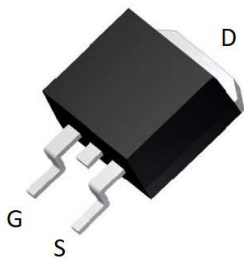
TO-263 top view
