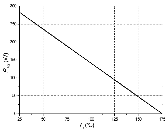
FIG.7: Power derating
