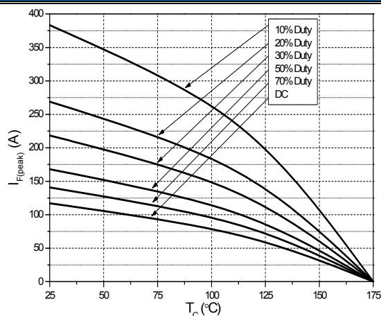
FIG.8: Current derating
