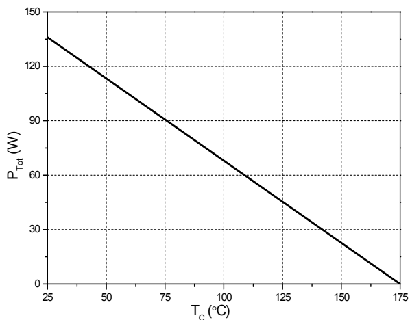
FIG.7: Power derating
