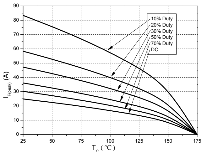
FIG.8: Current derating
