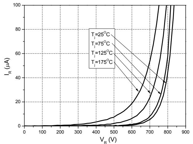
FIG.2: Reverse characteristics
