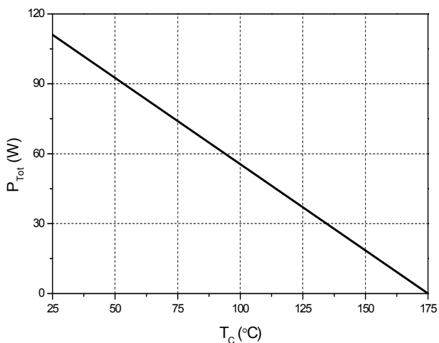
FIG.7: Power derating
