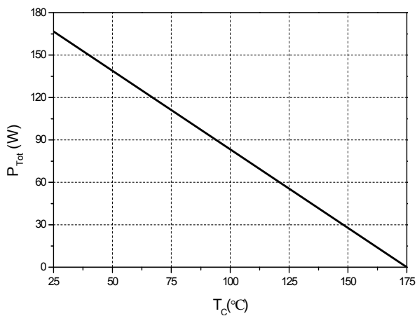
FIG.6: Power derating
