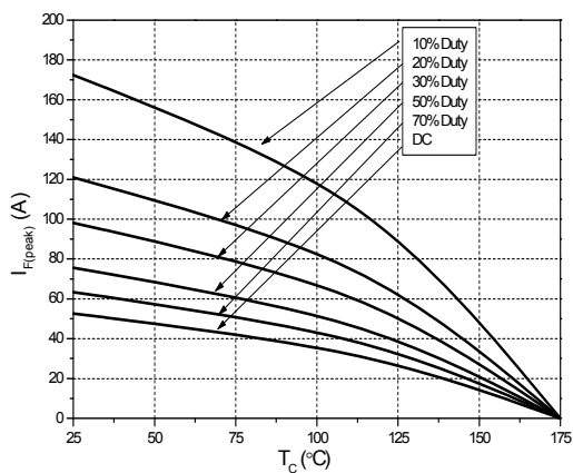
FIG.7: Current derating
