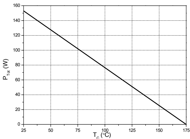
FIG.7: Power derating
