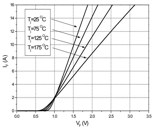
FIG.1: Forward characteristics
