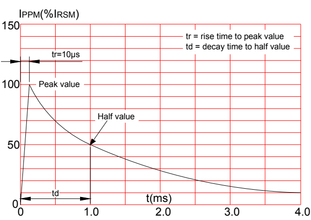
FIG.3: Pulse waveform
